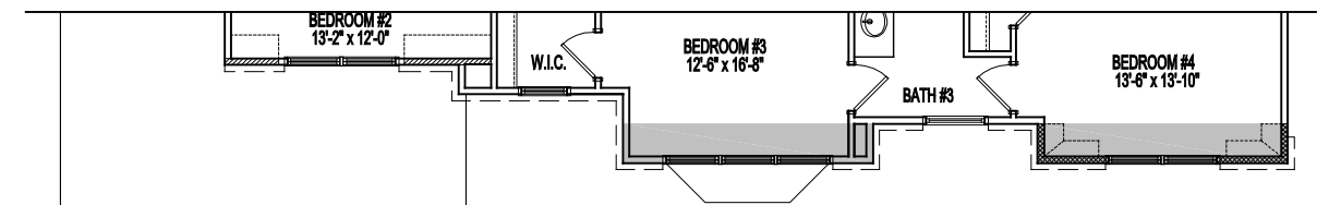
PARTIAL SECOND FLOOR PLAN ELEVATION 7A/B 02-03-23
