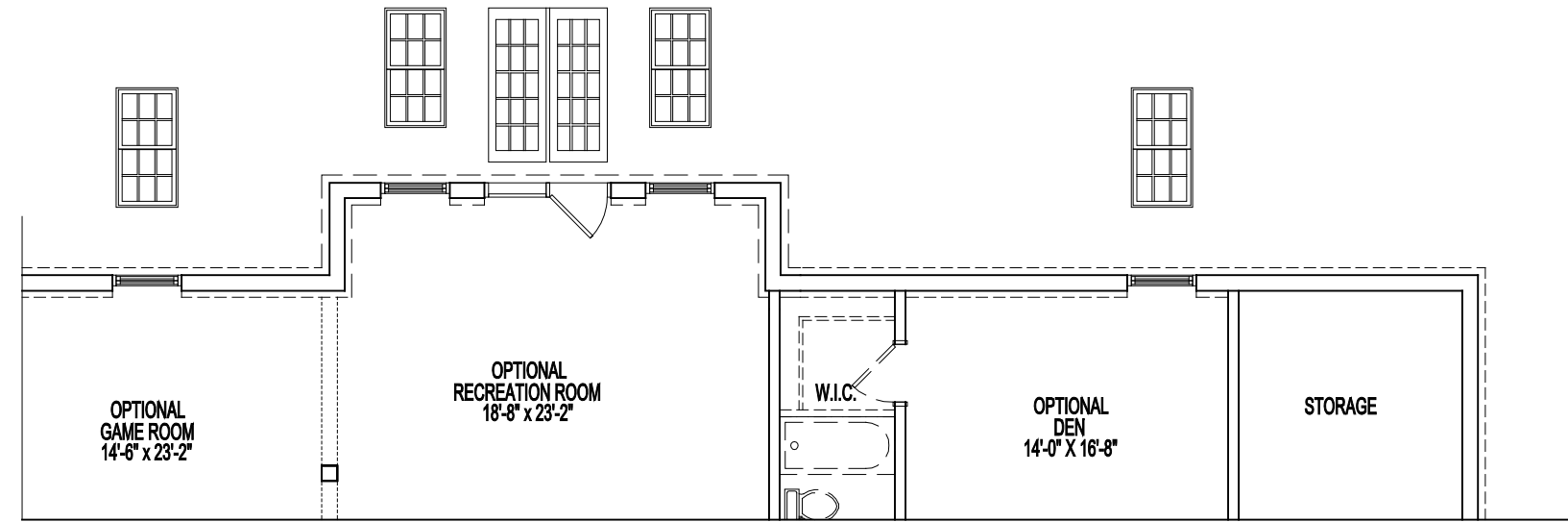
PARTIAL FOUNDATION / BASEMENT PLAN W/ WALKOUT
