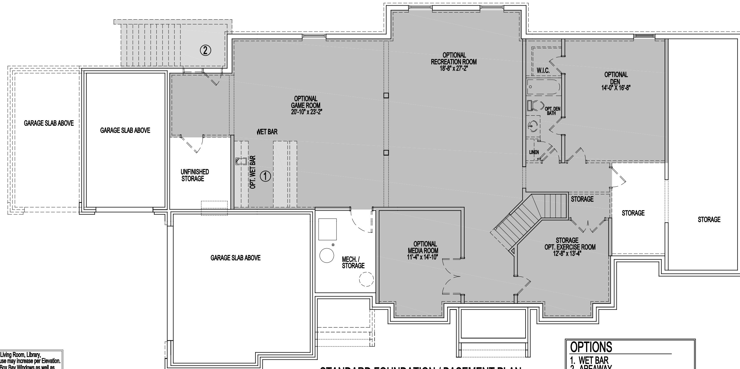
STANDARD FOUNDATION / BASEMENT PLAN
