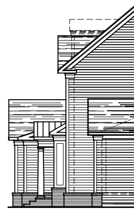
PARTIAL LEFT ELEVATION ELEVATION #1A 02-03-23
