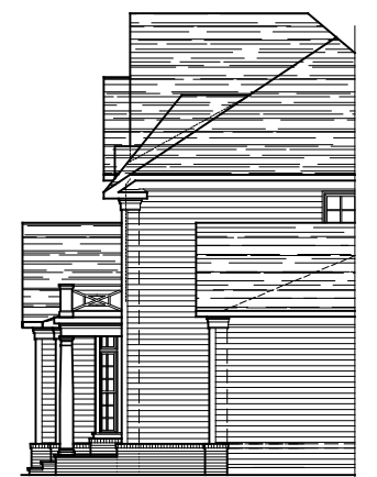
PARTIAL LEFT ELEVATION ELEVATION #7B 02-03-23
