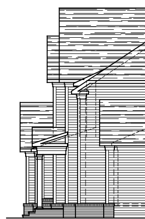
PARTIAL LEFT ELEVATION ELEVATION #8A 02-03-23
