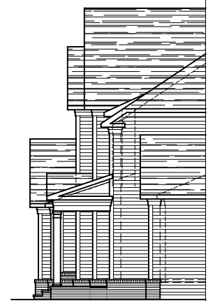
PARTIAL LEFT ELEVATION ELEVATION #8B 02-03-23
