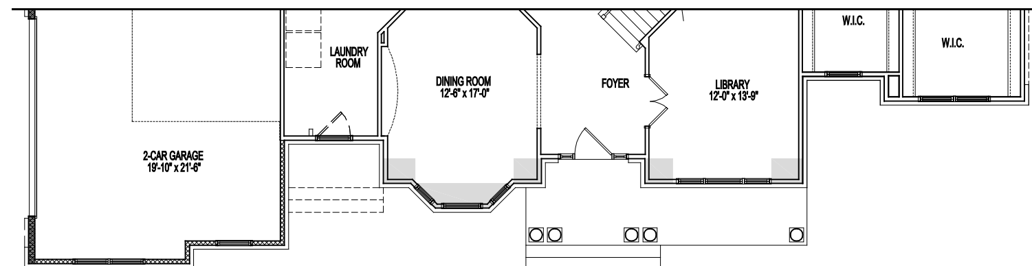
PARTIAL FIRST FLOOR PLAN ELEVATION 7B 02-03-23
