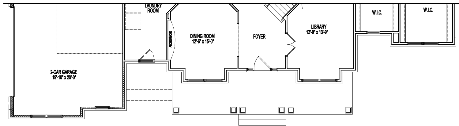
PARTIAL FIRST FLOOR PLAN ELEVATION 3B 02-03-23
