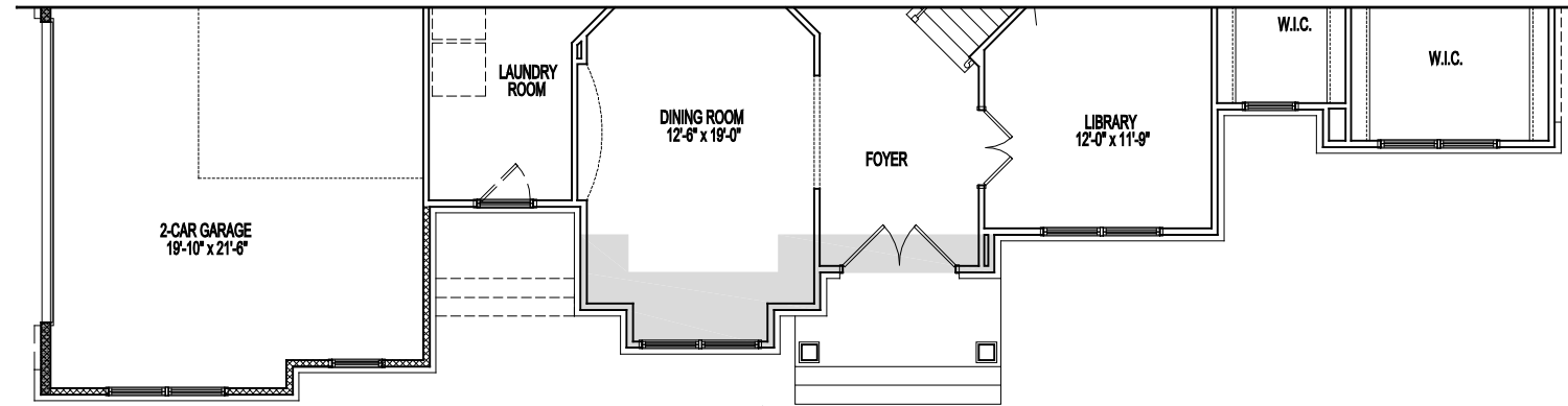
PARTIAL FIRST FLOOR PLAN ELEVATION 8A 02-03-23
