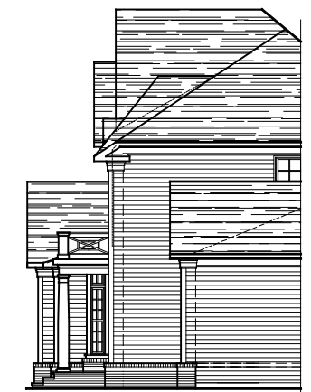
PARTIAL LEFT ELEVATION ELEVATION #7A 02-03-23
