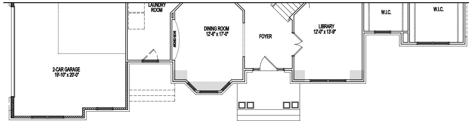
PARTIAL FIRST FLOOR PLAN ELEVATION 6A 02-03-23
