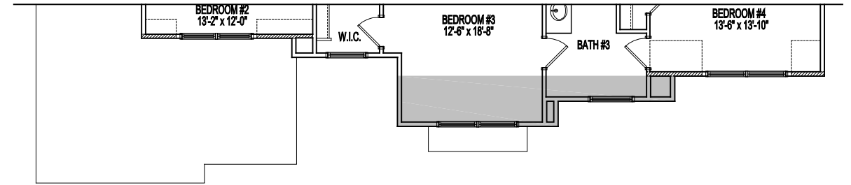
PARTIAL SECOND FLOOR PLAN ELEVATION 8A/B 02-03-23
