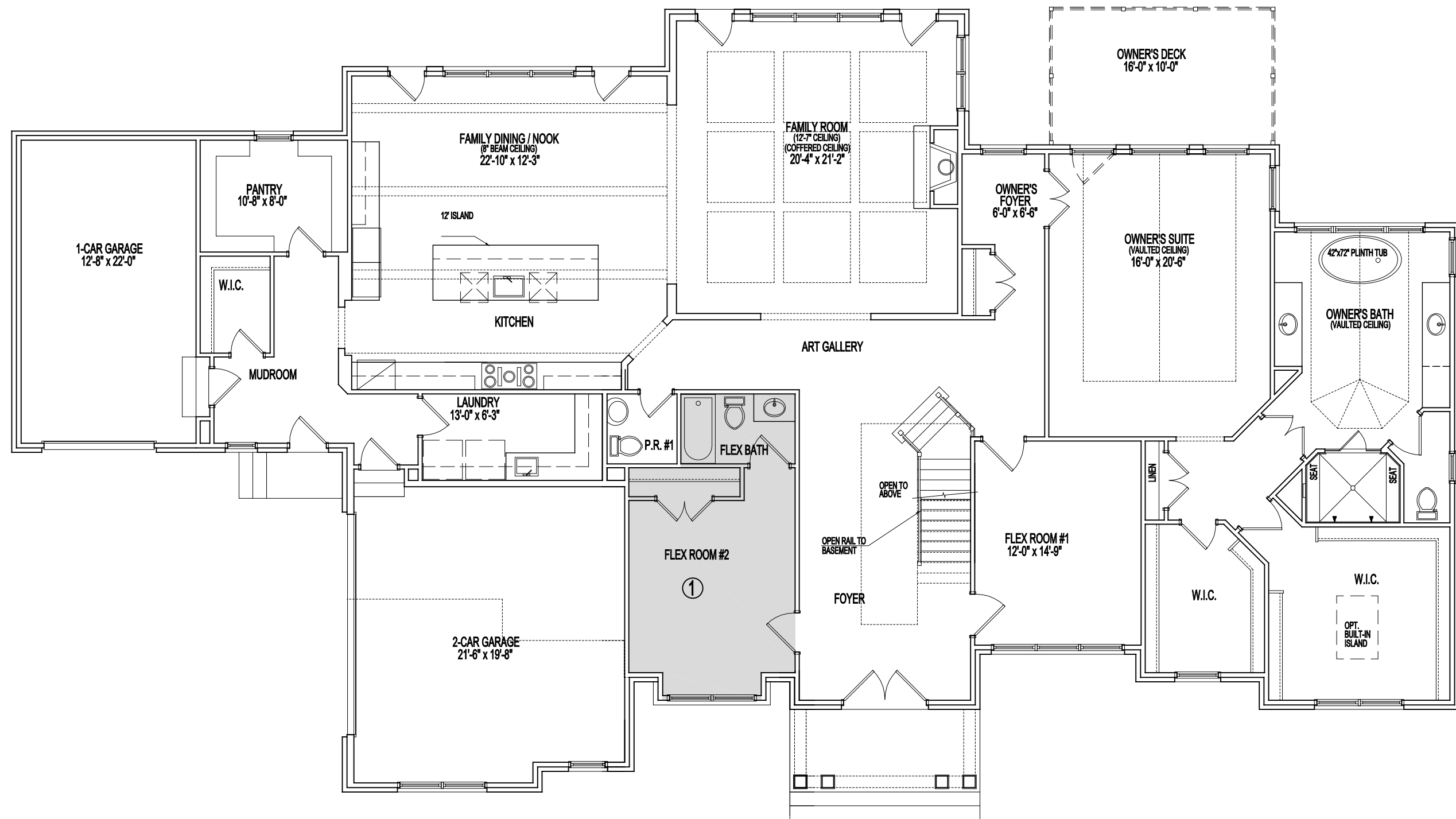
PARTIAL FIRST FLOOR PLAN
