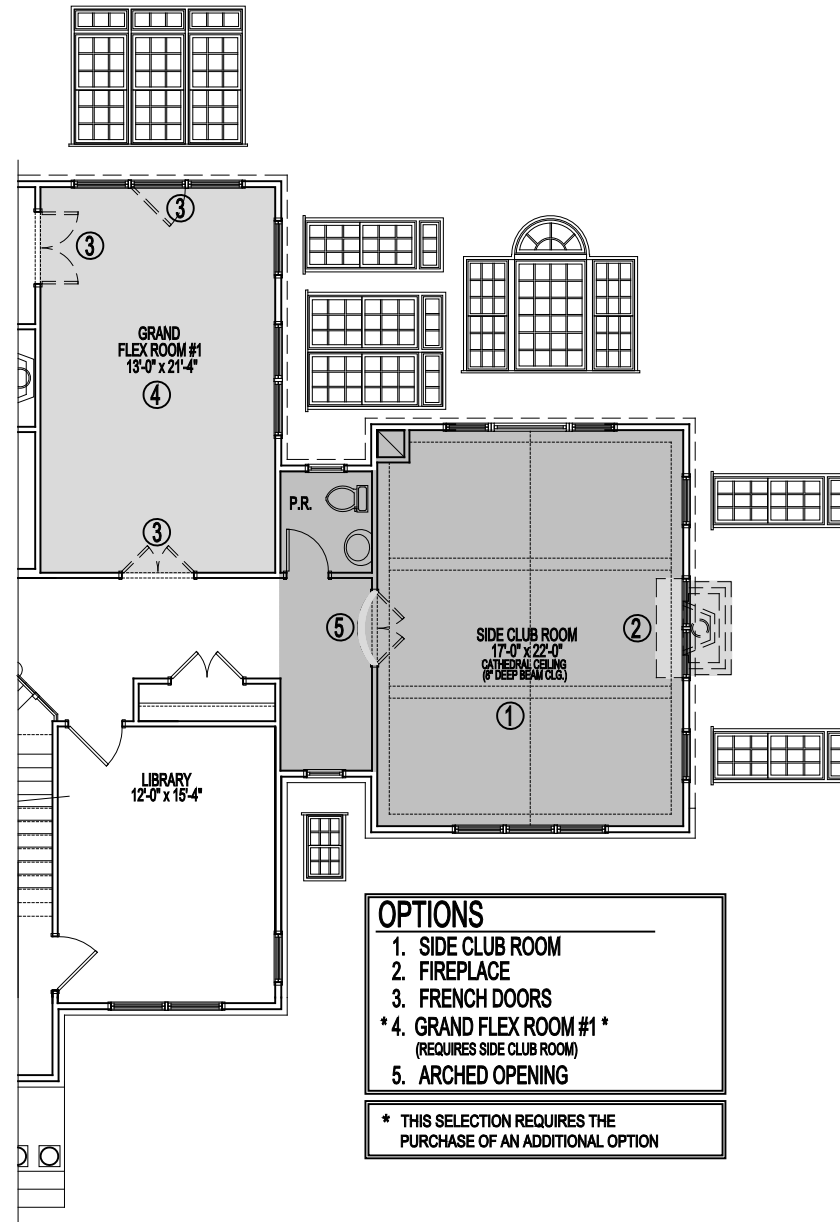
PARTIAL FIRST FLOOR PLAN
