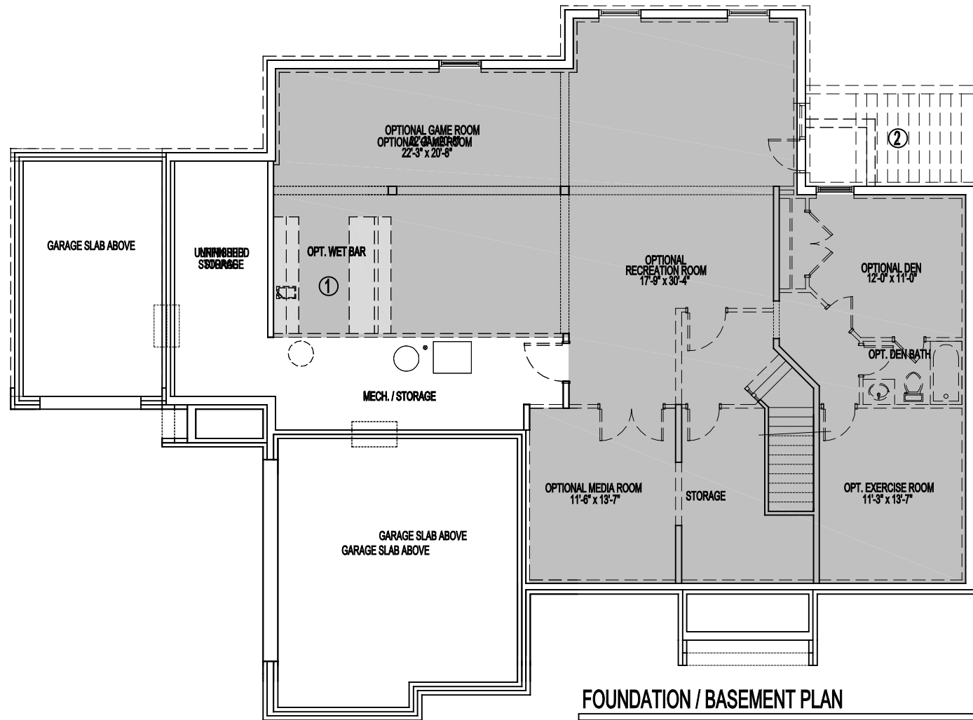
PARTIAL FOUNDATION / BASEMENT PLAN W/ WALKOUT 06-09-22 WINDOW LOCATIONS MAY VARY DUE TO GRADE
