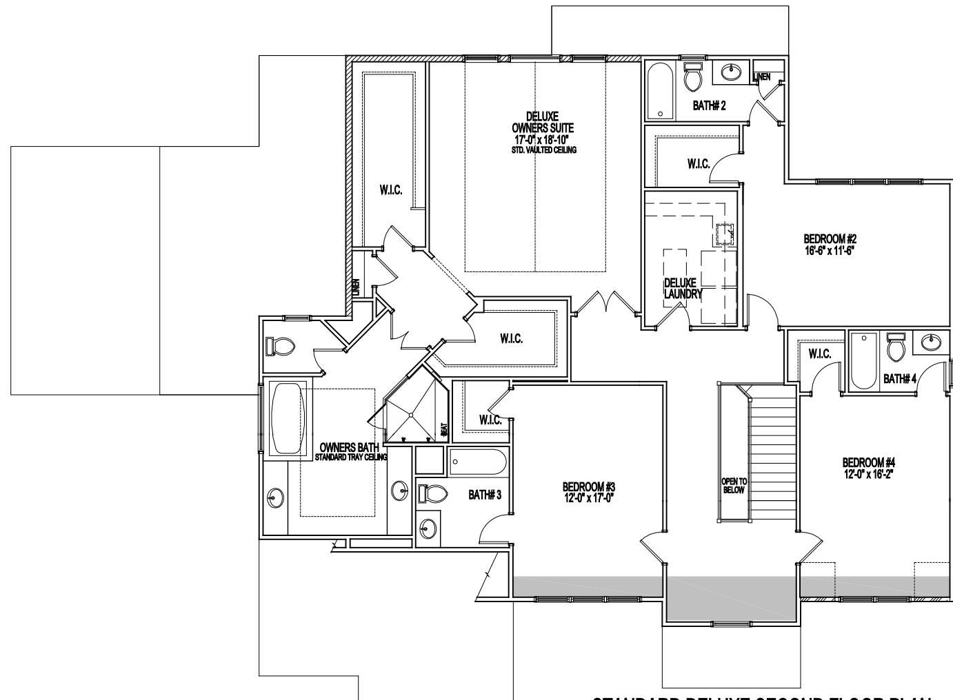
STANDARD DELUXE SECOND FLOOR PLAN
