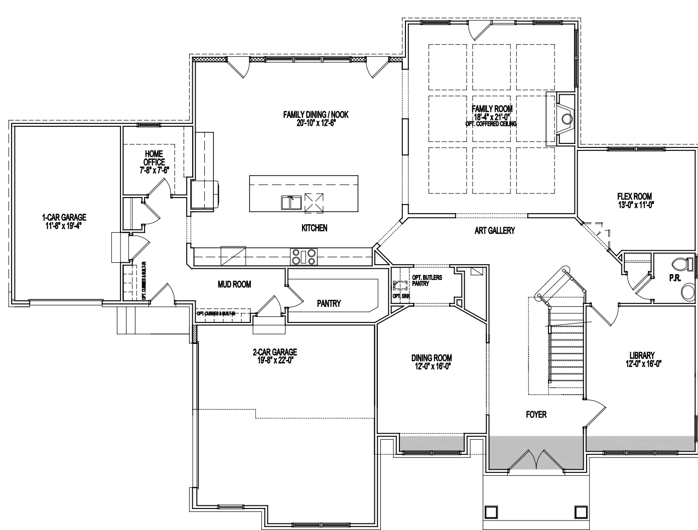
FIRST FLOOR PLAN SHOWN W/ ELEVATION 12A 06-09-22
