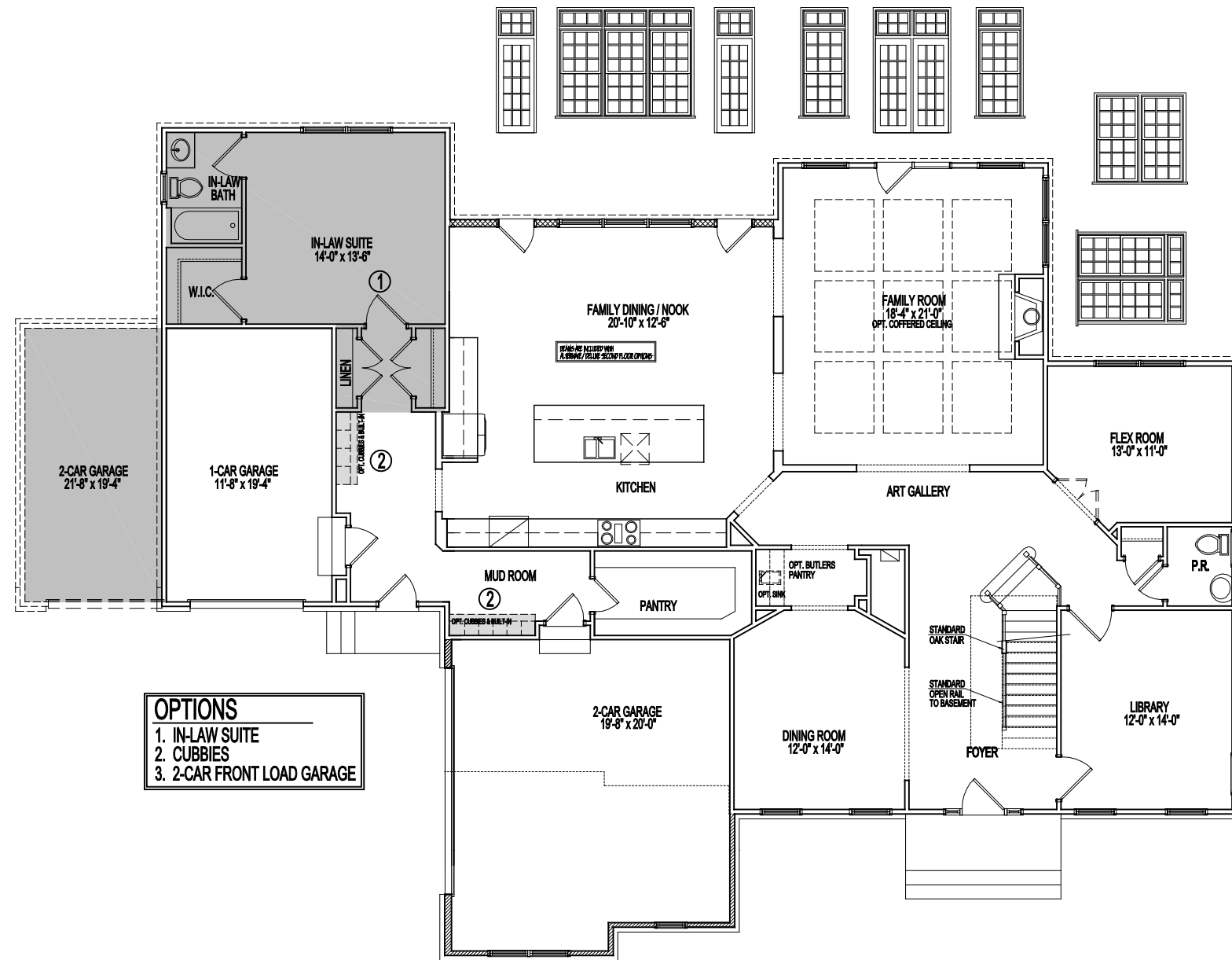
FIRST FLOOR PLAN 06-09-22
