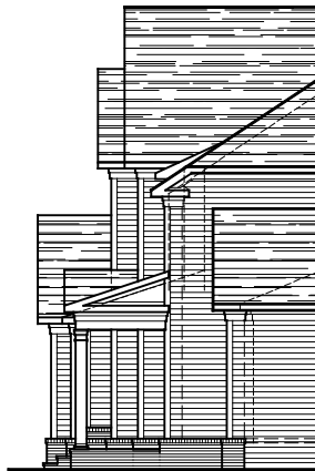
PARTIAL LEFT ELEVATION ELEVATION #8B 02-03
