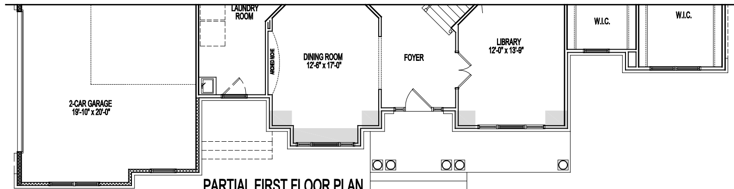
PARTIAL FIRST FLOOR PLAN ELEVATION 5B 02-03-23
