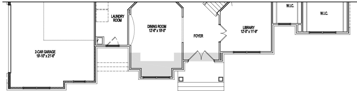
PARTIAL FIRST FLOOR PLAN ELEVATION 8A 02-03-23
