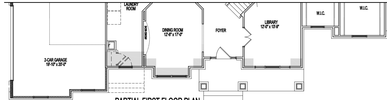
PARTIAL FIRST FLOOR PLAN ELEVATION 4B 02-03-23
