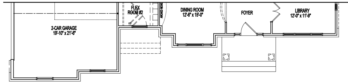
PARTIAL FIRST FLOOR PLAN ELEVATION #2 & 2A 04-06-22
