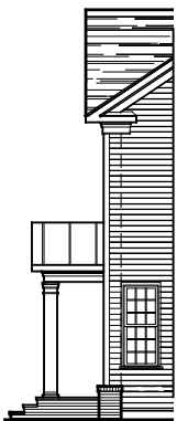
PARTIAL RIGHT SIDE ELEVATION ELEVATION #1A 02-04-22
