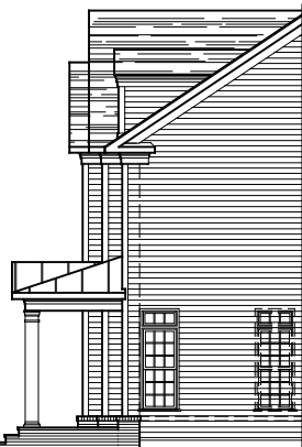
PARTIAL RIGHT SIDE ELEVATION ELEVATION #6B 02-04-22
