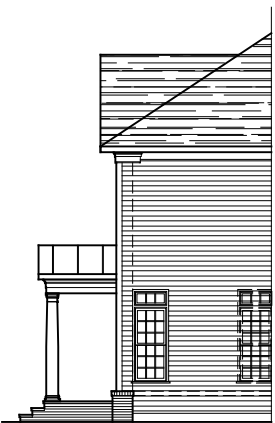
PARTIAL RIGHT SIDE ELEVATION ELEVATION #4A 02-04-22
