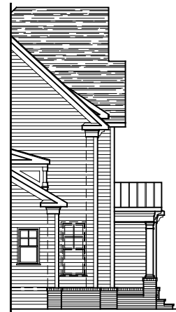
PARTIAL LEFT SIDE ELEVATION ELEVATION #7A 02-04-22
