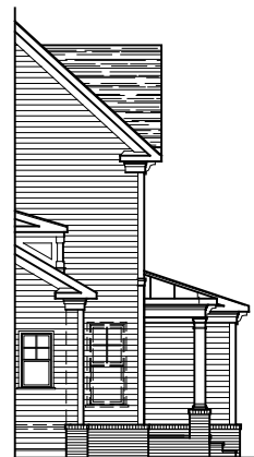
PARTIAL LEFT SIDE ELEVATION ELEVATION #3A 02-04-22
