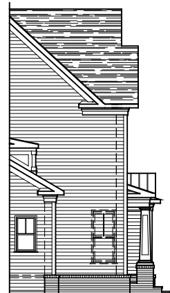
PARTIAL LEFT SIDE ELEVATION ELEVATION #4A 02-04-22
