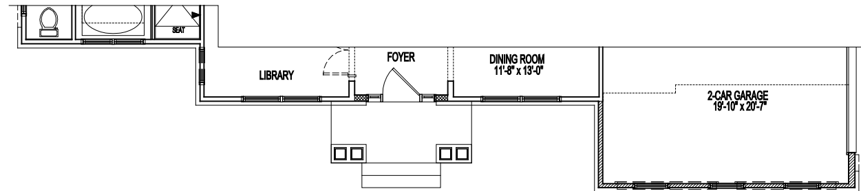
PARTIAL FIRST FLOOR PLAN ELEVATION #3A 02-04-22
