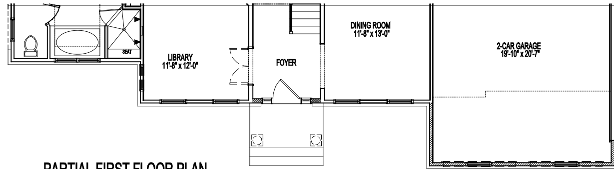
PARTIAL FIRST FLOOR PLAN ELEVATION #2A 02-04-22
