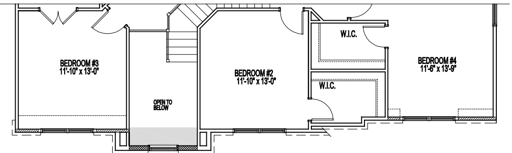
PARTIAL SECOND FLOOR PLAN ELEVATION #7A & 7B 02-04-22
