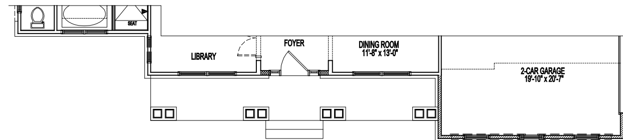
PARTIAL FIRST FLOOR PLAN ELEVATION #3B 02-04-22
