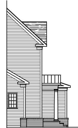
PARTIAL LEFT SIDE ELEVATION ELEVATION #2A 02-04-22
