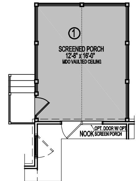
PARTIAL FIRST FLOOR PLAN
