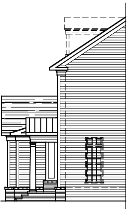
PARTIAL RIGHT ELEVATION ELEVATION #1A 07-16-21
