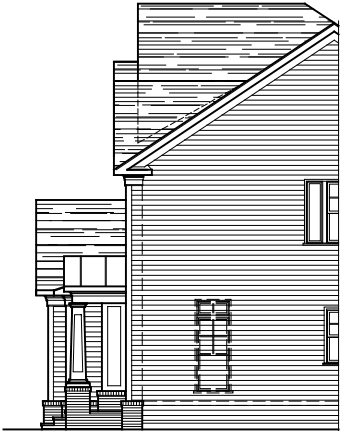
PARTIAL RIGHT ELEVATION ELEVATION #10A 07-16-21
