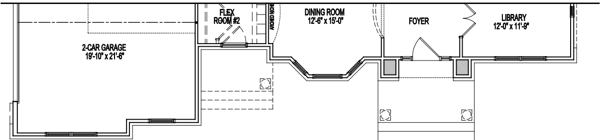
PARTIAL FIRST FLOOR PLAN ELEVATION #4 & 4A 07-16-21
