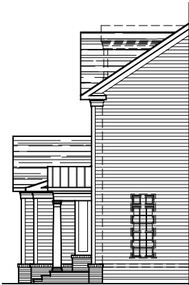
PARTIAL RIGHT ELEVATION ELEVATION #2A 07-16-21
