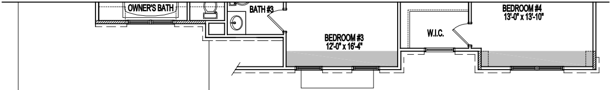
PARTIAL SECOND FLOOR PLAN ELEVATION #10A & 10B 07-16-21
