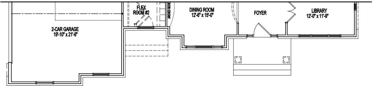
PARTIAL FIRST FLOOR PLAN ELEVATION #2 & 2A 07-16-21
