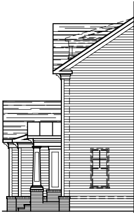
PARTIAL RIGHT ELEVATION ELEVATION #3A 07-16-21
