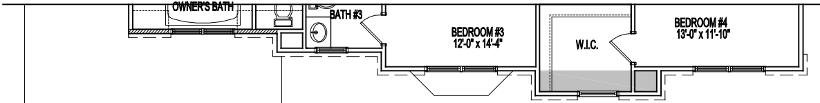
PARTIAL SECOND FLOOR PLAN ELEVATION #4 & 4A 07-16-21
