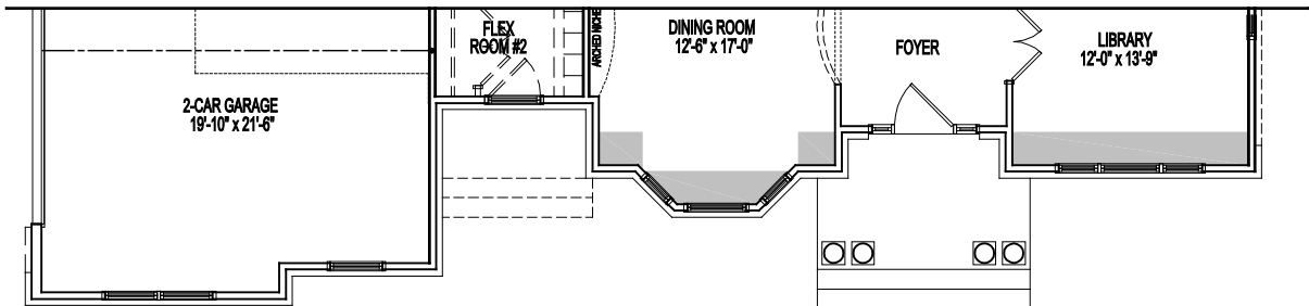
PARTIAL FIRST FLOOR PLAN ELEVATION #7A 07-16-21
