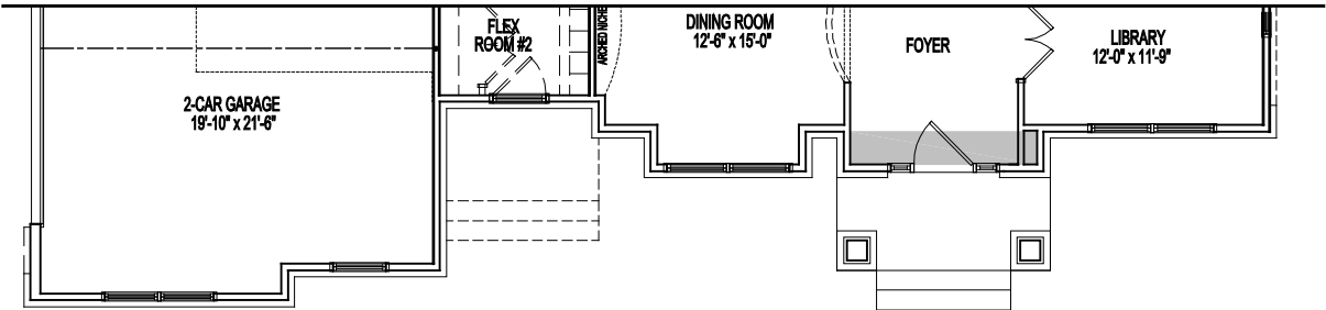
PARTIAL FIRST FLOOR PLAN ELEVATION #5A 07-16-21
