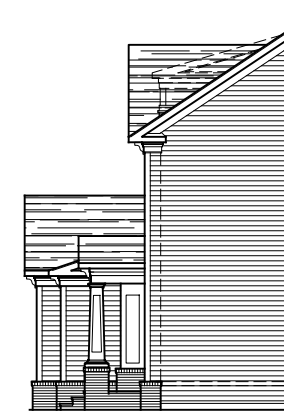
PARTIAL RIGHT ELEVATION ELEVATION #3A 04-01-2021
