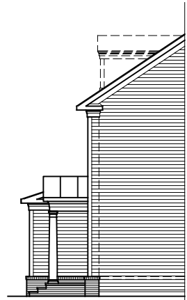
PARTIAL RIGHT ELEVATION ELEVATION #1A 04-01-2021
