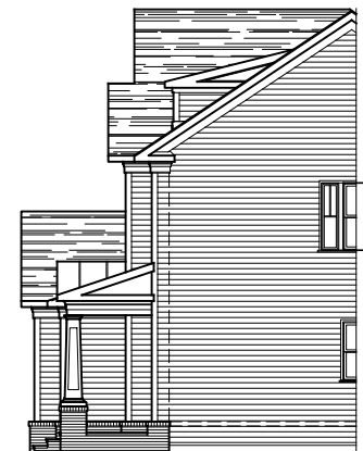
PARTIAL RIGHT ELEVATION ELEVATION #5B 04-01-2021
