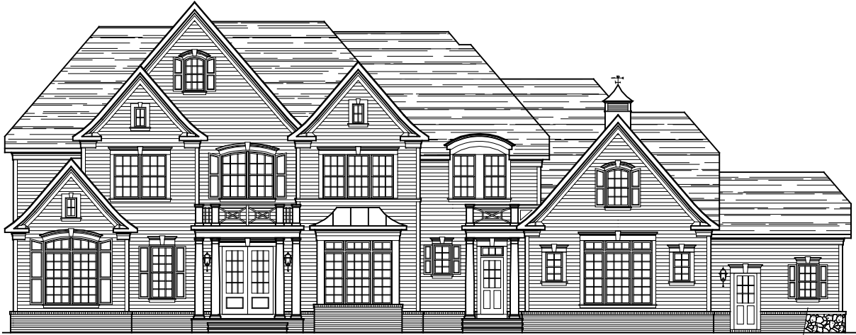
FRONT ELEVATION ELEVATION #7A
