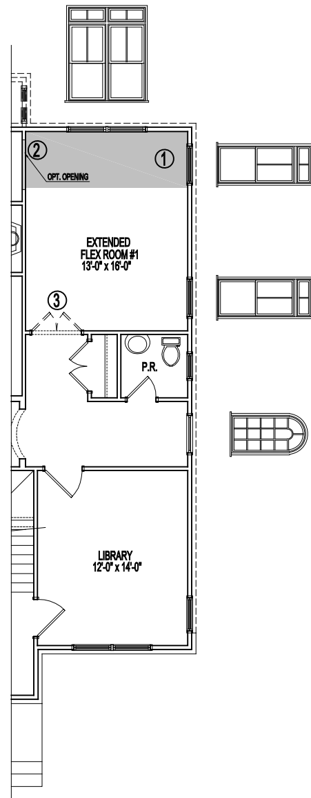
PARTIAL FIRST FLOOR PLAN
