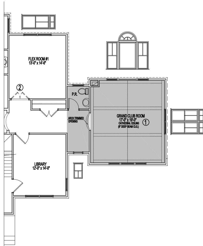
PARTIAL FIRST FLOOR PLAN 08-17-21
