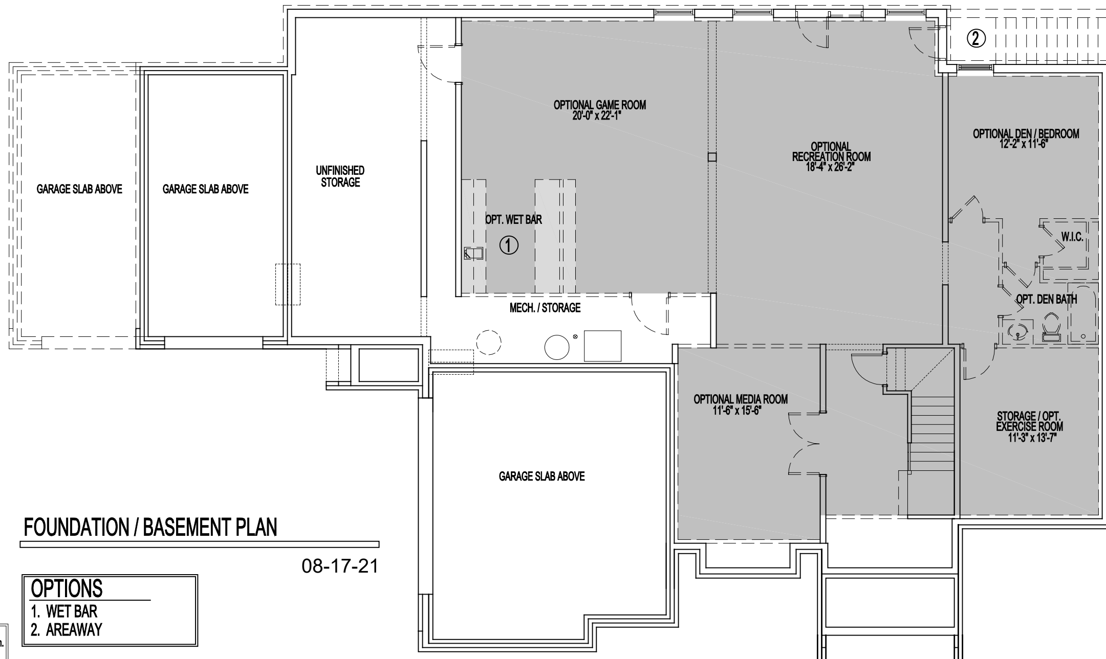
FOUNDATION / BASEMENT PLAN W/ WALKOUT
