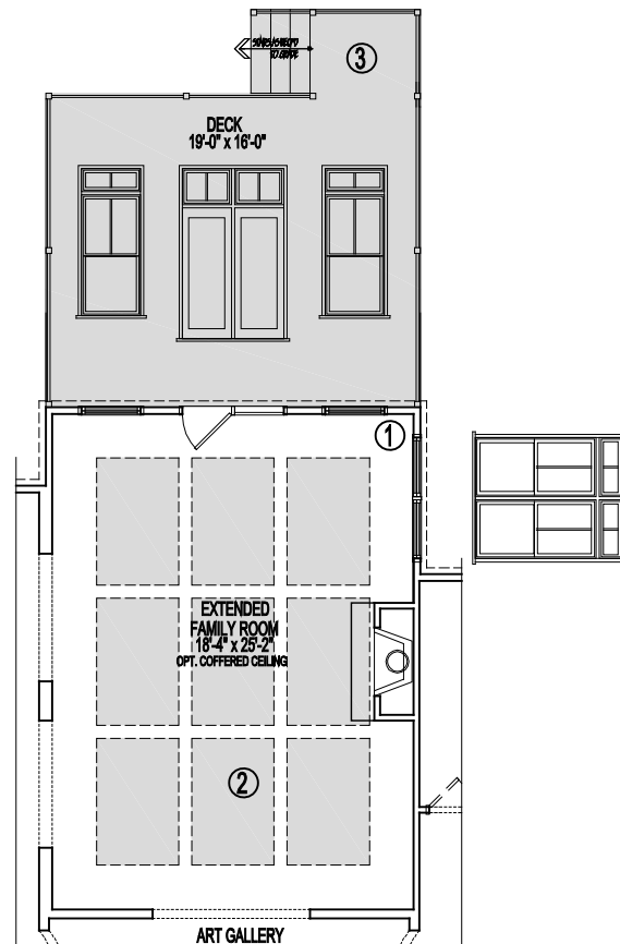
PARTIAL FIRST FLOOR PLAN
