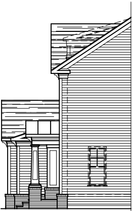
PARTIAL RIGHT ELEVATION ELEVATION #3A 07-16-21
