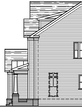
PARTIAL RIGHT ELEVATION ELEVATION #5A 07-16-21
