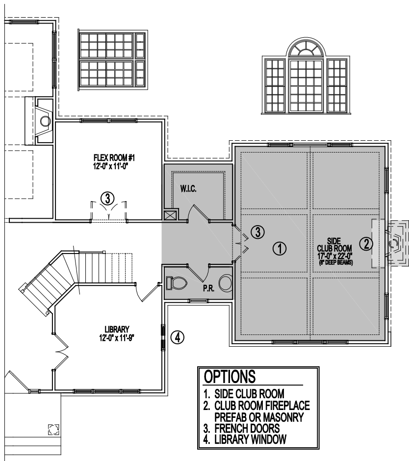
PARTIAL FIRST FLOOR PLAN 07-16-21
