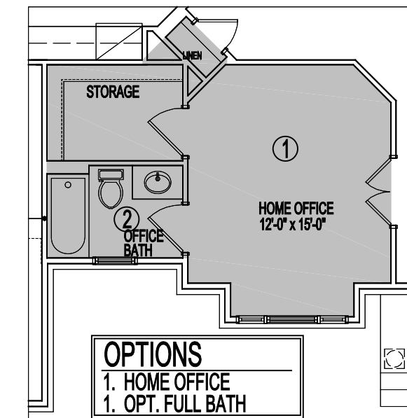
PARTIAL FIRST FLOOR PLAN
