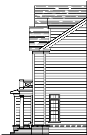
PARTIAL RIGHT SIDE ELEVATION ELEVATION #4A 08-29-19
