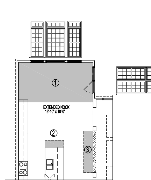
PARTIAL FIRST FLOOR PLAN
