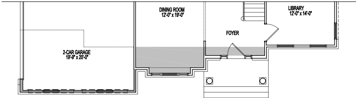
PARTIAL FIRST FLOOR PLAN ELEVATION 3A 08-29-19
