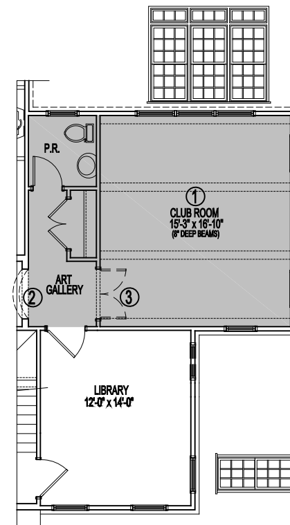
PARTIAL FIRST FLOOR PLAN
