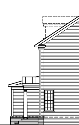
PARTIAL RIGHT SIDE ELEVATION
