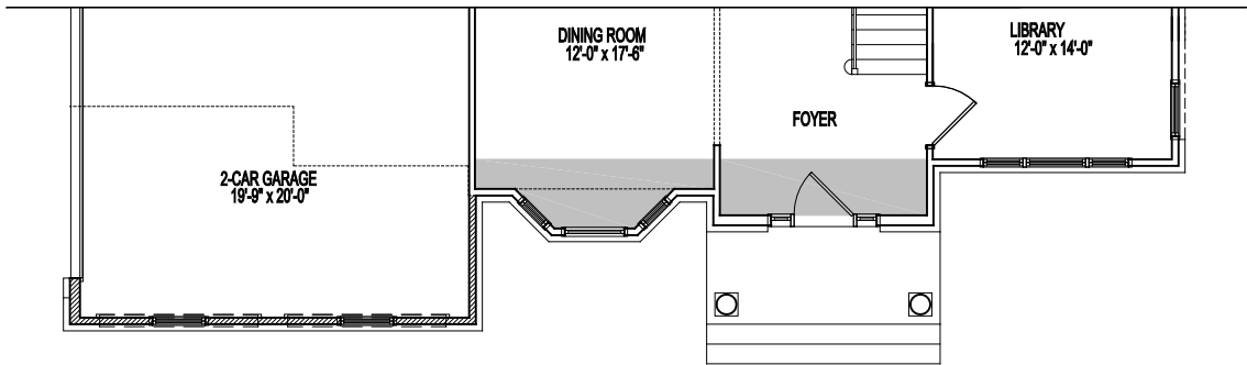
PARTIAL FIRST FLOOR PLAN ELEVATION 4A 08-29-19
