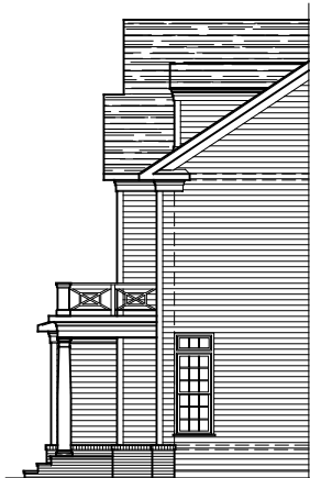
PARTIAL RIGHT SIDE ELEVATION ELEVATION #4B 08-29-19
