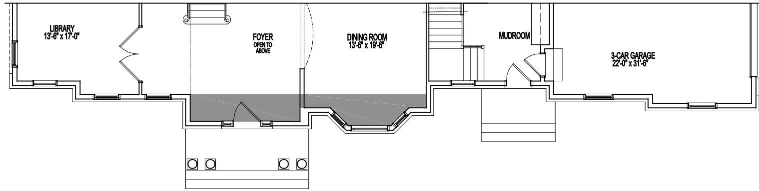
PARTIAL SECOND FLOOR PLAN ELEVATION #2A 08-29-19
