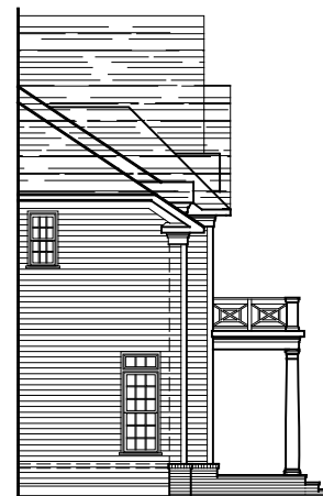
PARTIAL LEFT SIDE ELEVATION ELEVATION #5B 08-29-19
