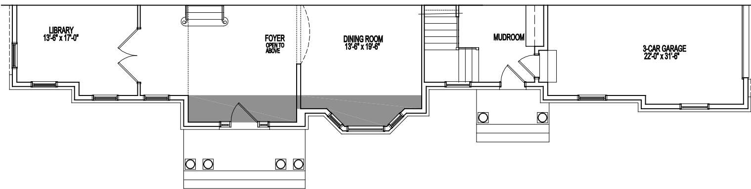
PARTIAL FIRST FLOOR PLAN ELEVATION #3A/B 08-29-19
