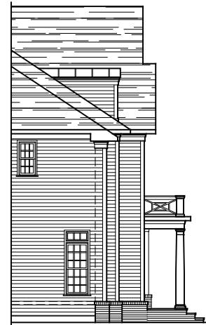
PARTIAL LEFT SIDE ELEVATION ELEVATION #3A 08-29-19
