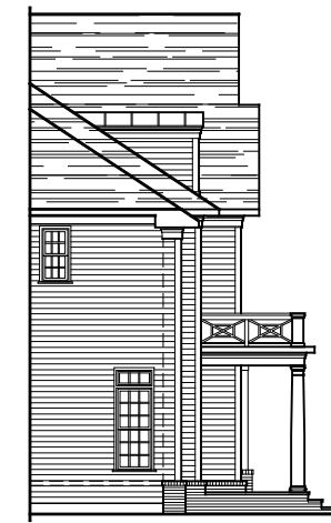
PARTIAL LEFT SIDE ELEVATION ELEVATION #3B 08-29-19
