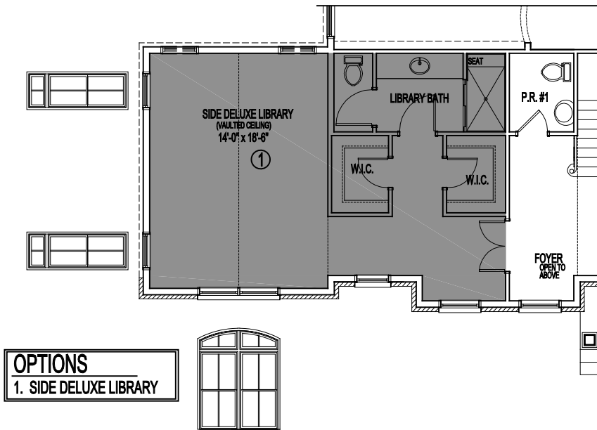
PARTIAL FIRST FLOOR PLAN ELEVATION #7A 08-29-19
