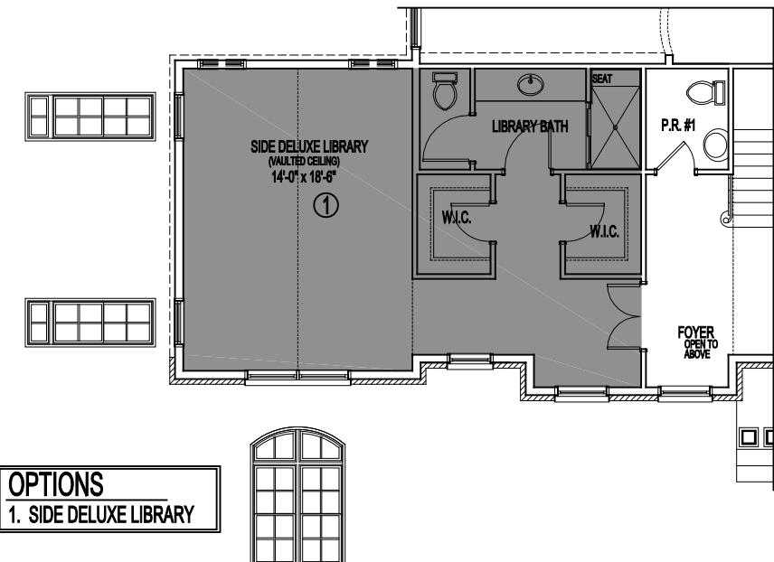
PARTIAL FIRST FLOOR PLAN ELEVATION #8A 08-29-19
