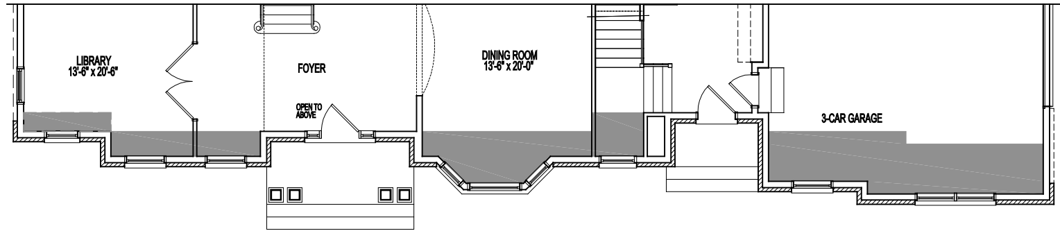
PARTIAL FIRST FLOOR PLAN
