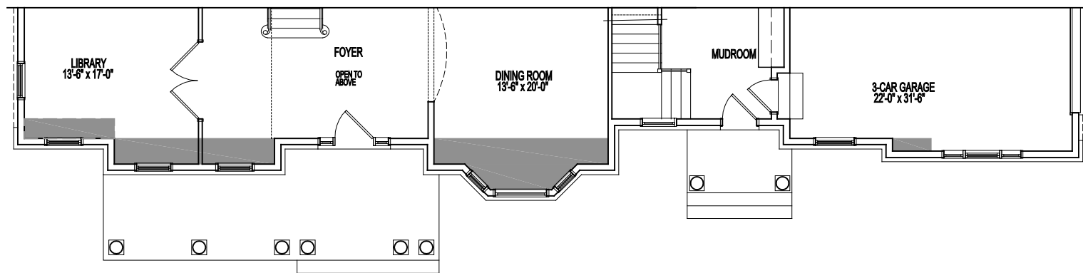
PARTIAL FIRST FLOOR PLAN ELEVATION #5A/B 08-29-19
