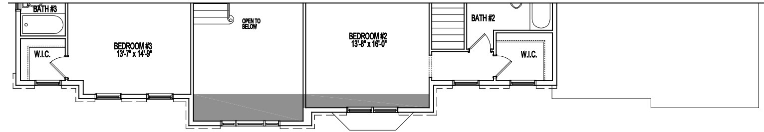
PARTIAL SECOND FLOOR PLAN ELEVATION #2A 08-29-19
