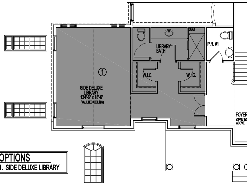
PARTIAL FIRST FLOOR PLAN ELEVATION #2B 08-29-19
