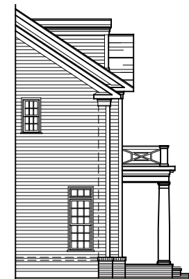
PARTIAL LEFT SIDE ELEVATION ELEVATION #1B 08-29-19
